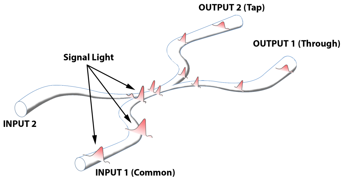
Coupling of Light on FUSED BICONICALLY TAPERED COUPLER
